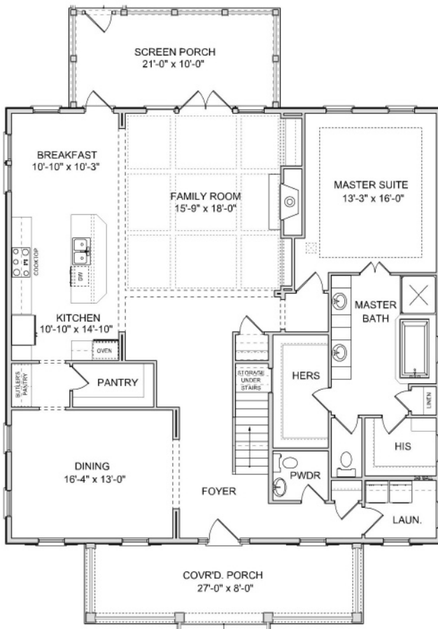
MAIN LEVEL PLAN
