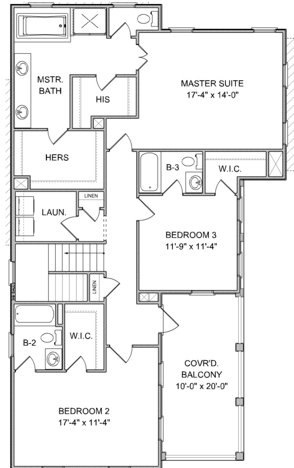
UPPER LEVEL
